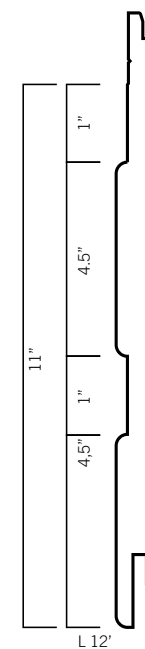
Profile Specification
